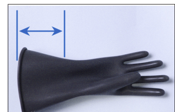
Figure 5– Insulated rubber gloves may be repaired, but only in the gauntlet area.
